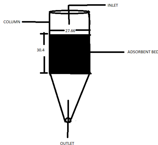
Fig 5: Adsorption Column
